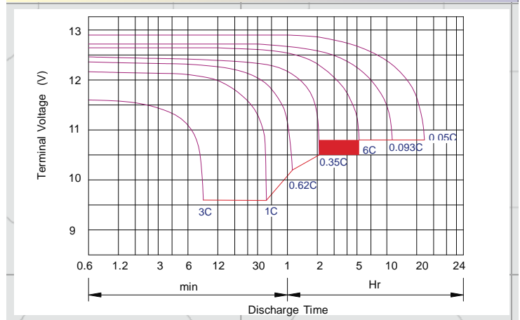
Discharge characteristic: GUVV
