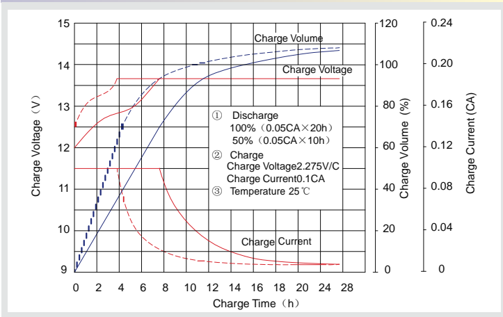
Charge characteristic: GUVV 100% standard use
